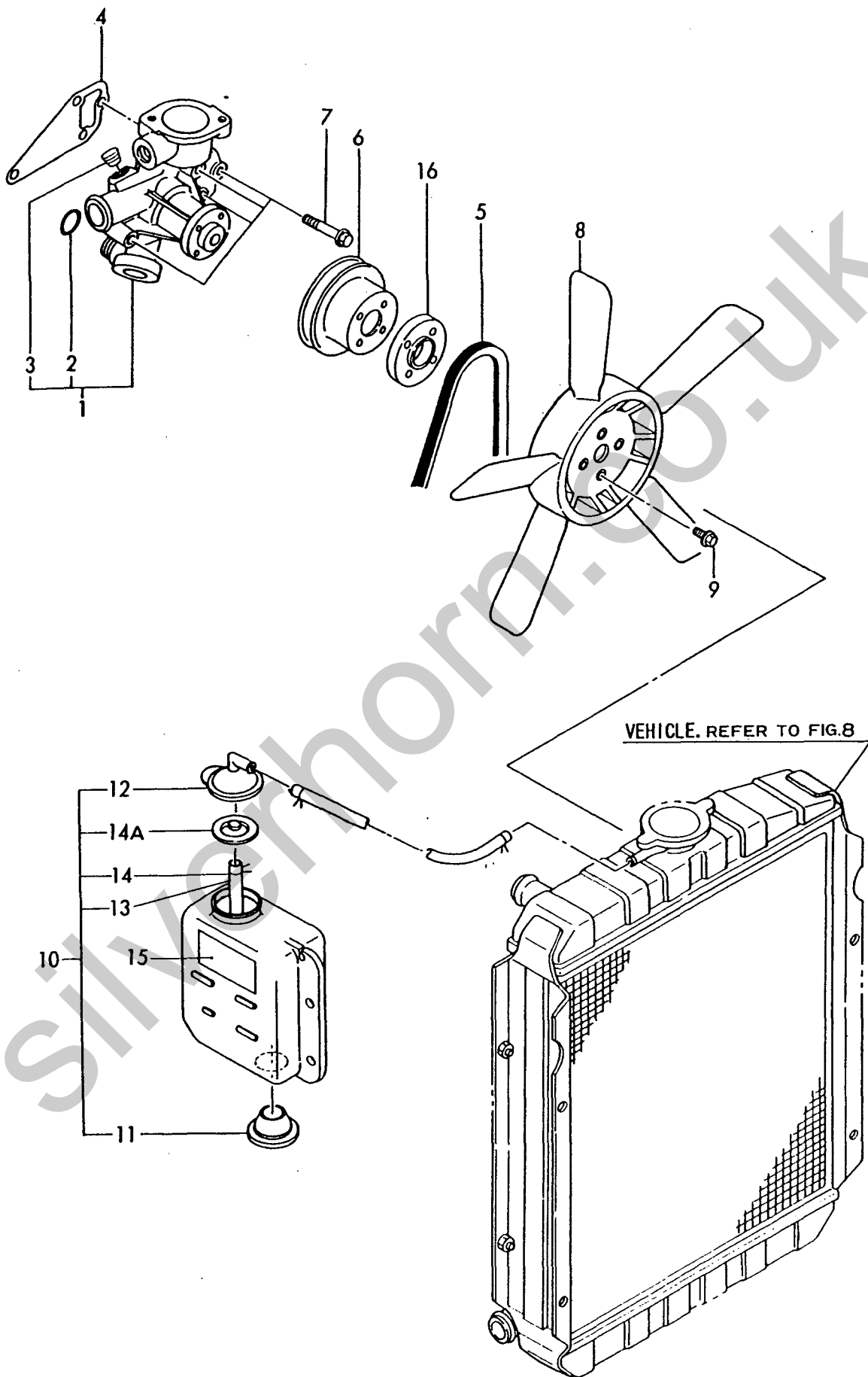
Fig. 21 CWポンプ COOLING WATER PUMP
